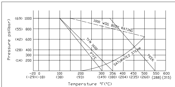
1/4"-4" SS Valve Sizes
