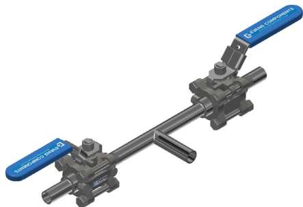
Double Horizontal Tee
