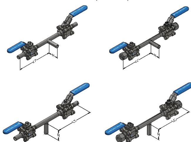
Double Horizontal/Vertical Tee (DHT/DVT)
